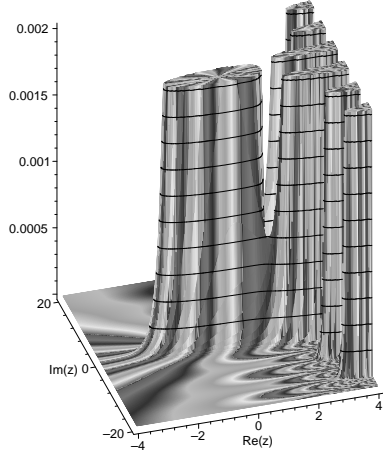
FIGURE 3. |S(z)/z^{11}|
