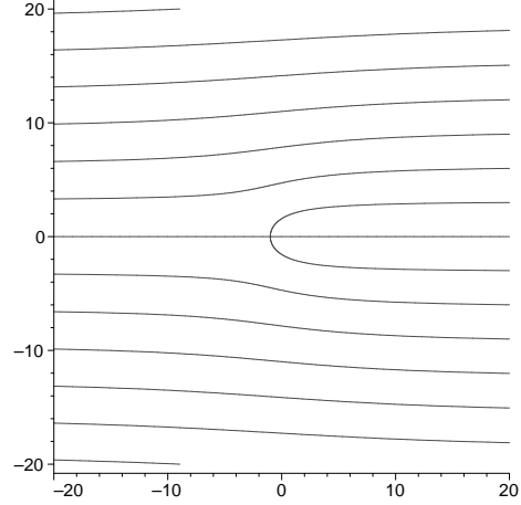
FIGURE 4. Stationary paths for S(z)
