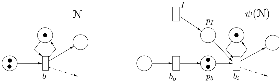
FIG. 9. Open Expansion of a Free Choice net.
