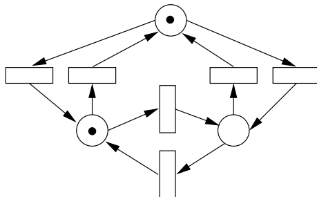
FIG. 2. A live and bounded S-net without any non-conflicting transition.
