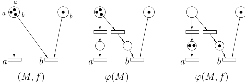
FIG. 14. The original net with pointed marking (M, f) (left) and the effect of \varphi .
