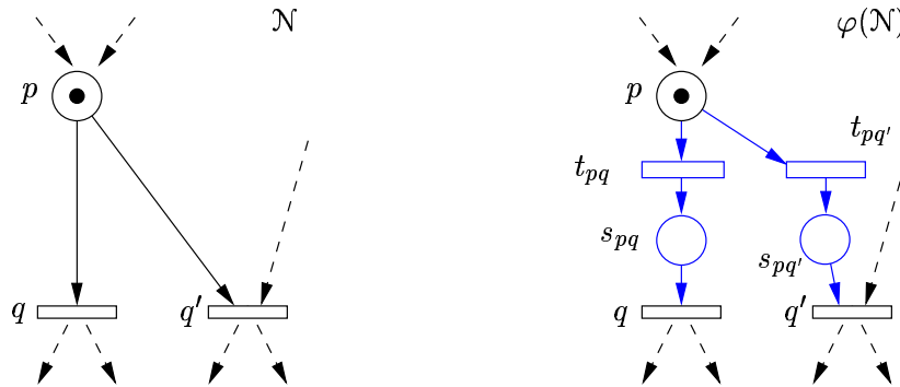
Figure 7: Free Choice expansion of a Petri net.
