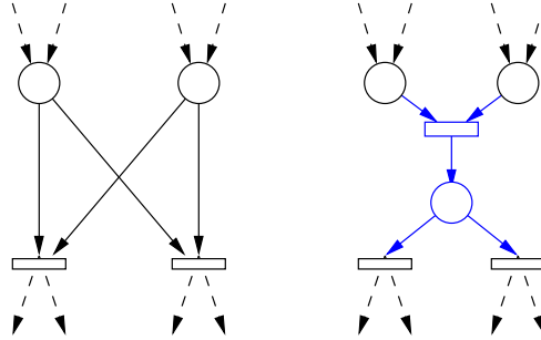
Figure 6: Transformation of an Extended Free Choice net into a Free Choice net.
