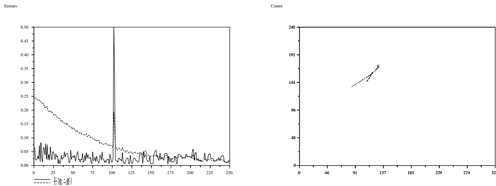
Figure 17: Pure translation: Errors (left) and image trajectory of the trihedron center (right).
