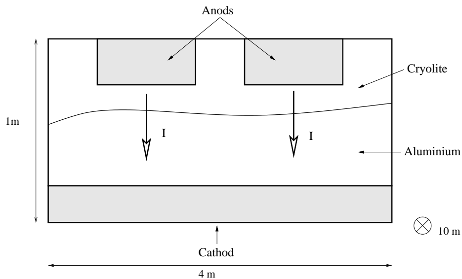
Figure 1: Schematic representation of an aluminium cell
