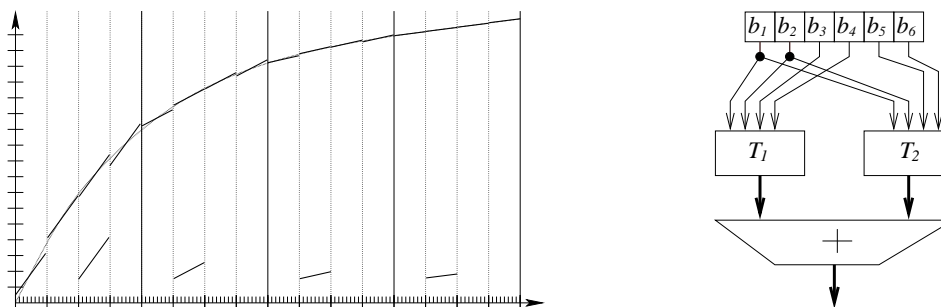
Figure 1: An example of bipartite approximation and architecture, for 6-bit input: w_I = 6 , \alpha = 4 , \gamma = 2 , \beta = 2 .
