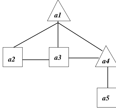
Figure 3: Example of graph with five nodes.
