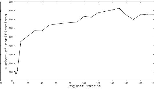
Figure 7: Network traffic with RTT=500ms
