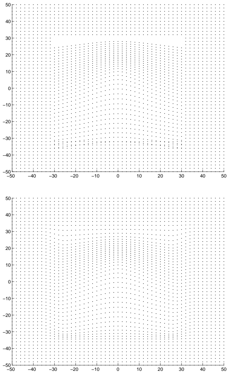
Figure 7: The application of the f function is restricted thanks to: top, a non-continuous function (a door function); bottom, a continuous function (the sine function presented in Section 3).
