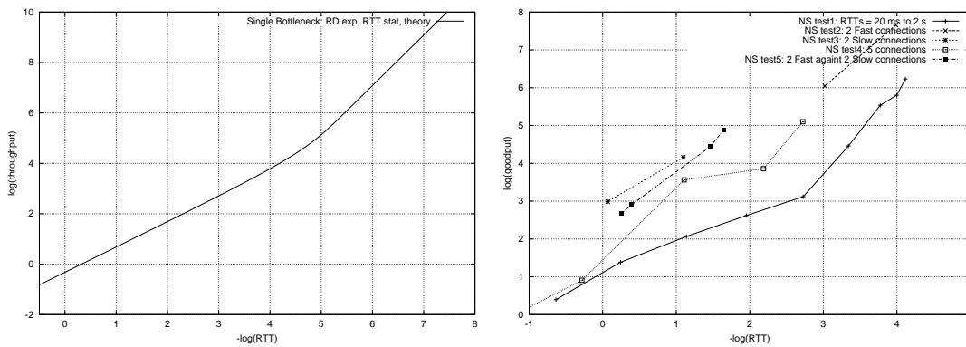
Figure 14: Left: Throughput vs RTTs in log-log as predicted by theory. Right: NS simulation of 5 different cases when varying parameters (number of flows, capacities, propagation delays).
