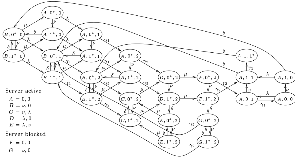
Figure 6: System states and transition rates in the centralized approach.
