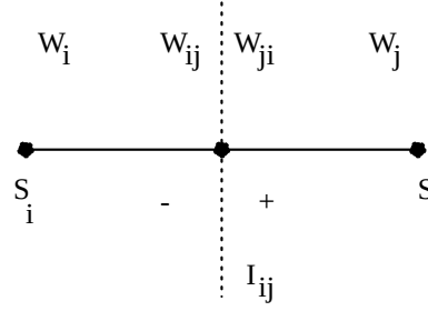
Figure 3: Position of W_{ij} and W_{ji} on [S_i, S_j]
