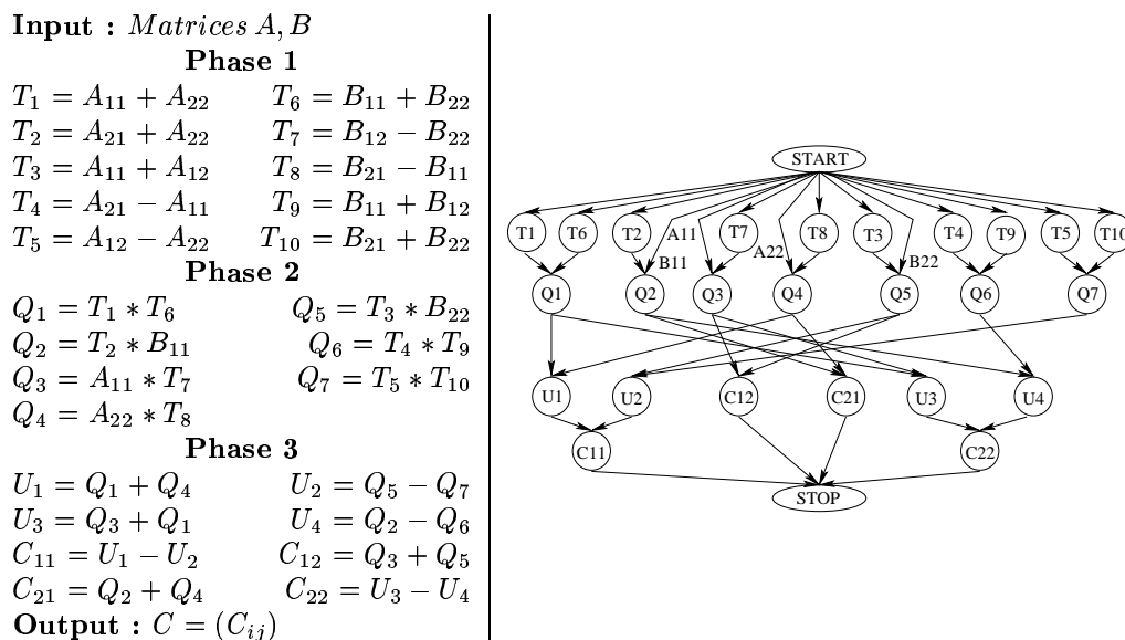
Figure 1: First level of recursion of Strassen algorithm (left) and its MDG representation (right).
