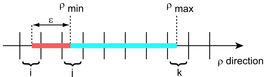
Figure 4: Rasterization in plane space.
