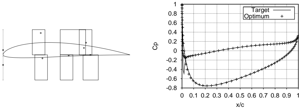
Figure 6: NACA4412 :
