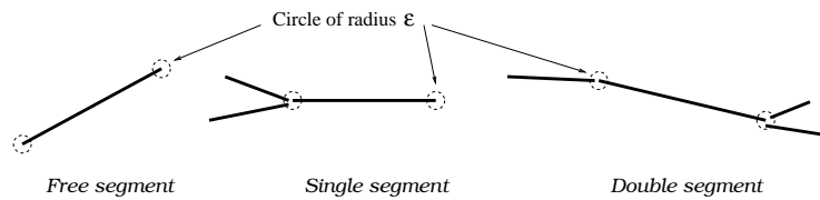
Figure 1: Segment types defined with respect to R_c .
