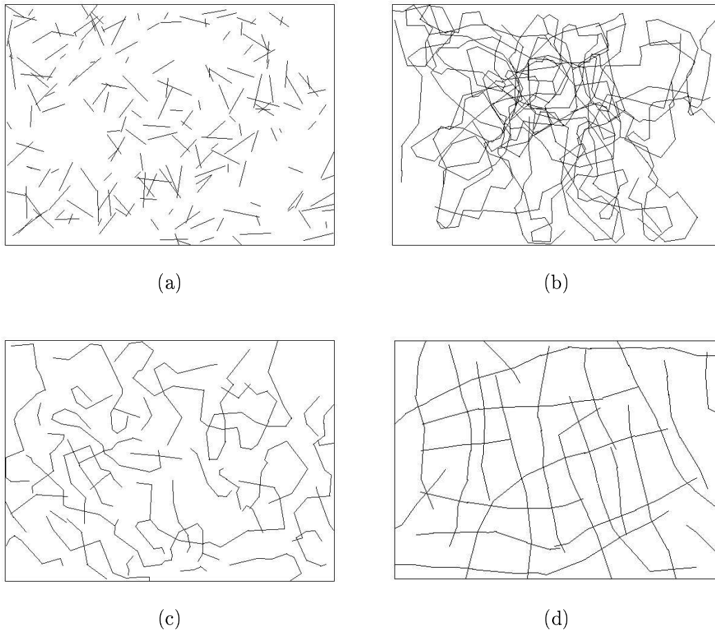
Figure 13: Samples of the "Quality Candy" Model - (a) Process without interaction : \omega_i = 0 \forall i - (b) Process only depending on segment states : \omega_f \neq 0, \omega_r \neq 0, \omega_c = 0 - (c) Process depending on segment states and on external bad orientation : \omega_c = 0 - (d) Complete model.
