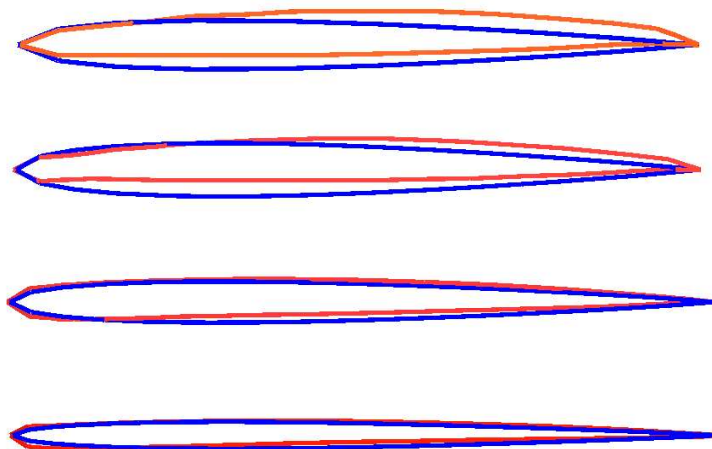
Figure 15: Isolated wings of the Supersonic Business Jet. Optimization Strategy I. Shape optimization shown at the four wing sections. From top to bottom: Sections A, B, C and D. In blue, the original shape.
