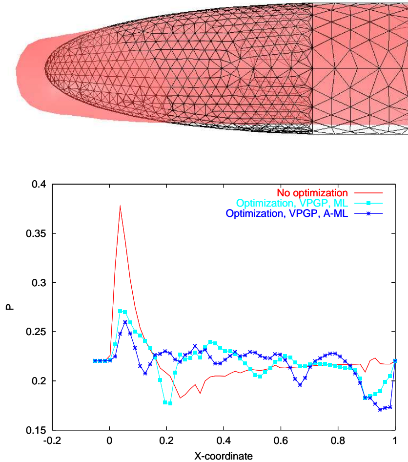
Figure 9: Aircraft's Generic Nose. Top, original geometry (mesh shown) and optimized shape (solid). Bottom, pressure along a centered line below.
