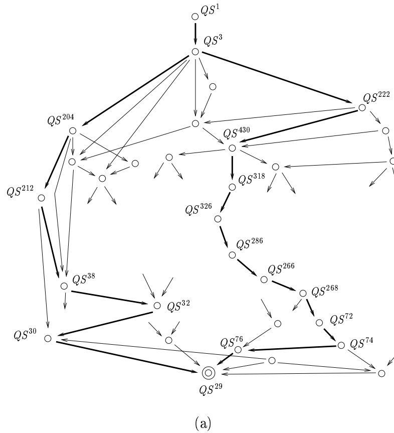
Figure 12: (a) Fragment of the state transition graph produced for vegetative growth conditions, when Signal is switched on ( \theta_s < u_s \leq max_s ). (b) Temporal evolution of selected protein concentrations in a typical qualitative behavior leading to the spo^+ phenotype. (c) Idem, but for a typical qualitative behavior leading to the spo^- phenotype.
