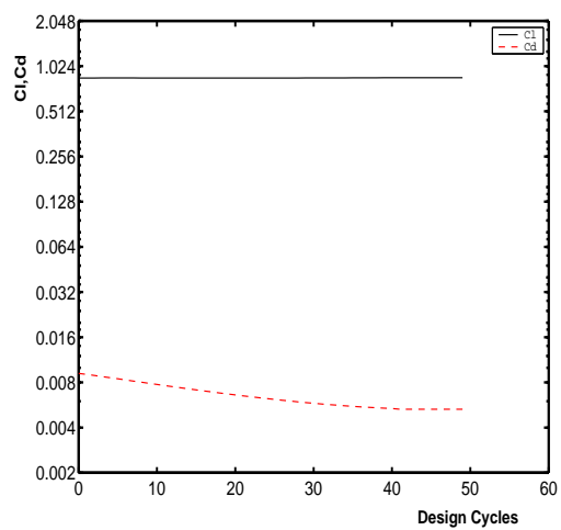
Figure 9: Drag and constraint histories
