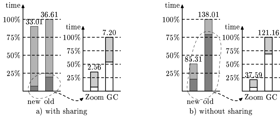
Figure 9: ASF+SDF Compiler
