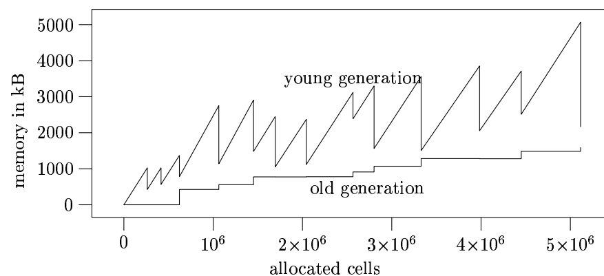
Figure 12: ASF+SDF Compiler (with sharing)
