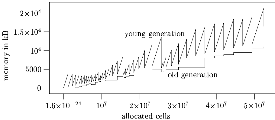
Figure 11: 32 th Fibonacci number (without sharing)
