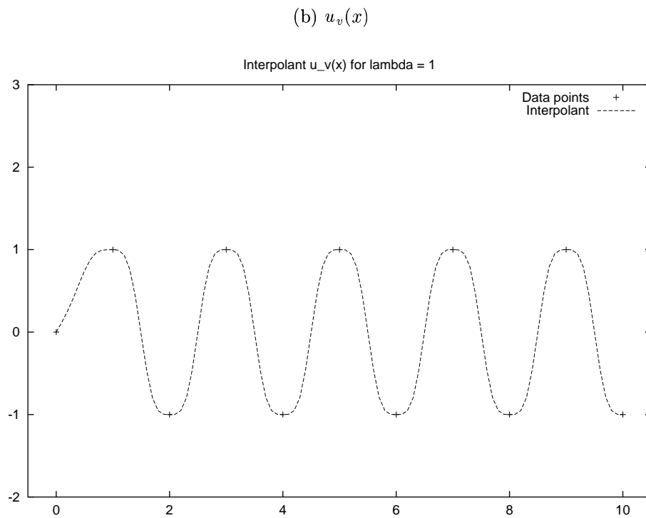
Figure 4: Behavior of the interpolants u_\lambda(x) of (78) and u_v(x) of (94) in the particular case of the sequence \{u_n\} given by (130); \lambda = 1 , \epsilon = 0.01 .
