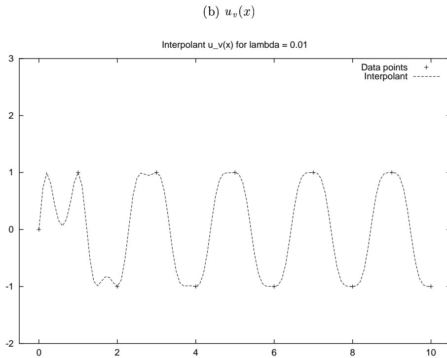
Figure 2: Behavior of the interpolants u_\lambda(x) of (78) and u_v(x) of (94) in the particular case of the sequence \{u_n\} given by (130); \lambda = 0.01 , \epsilon = 0.01 .
