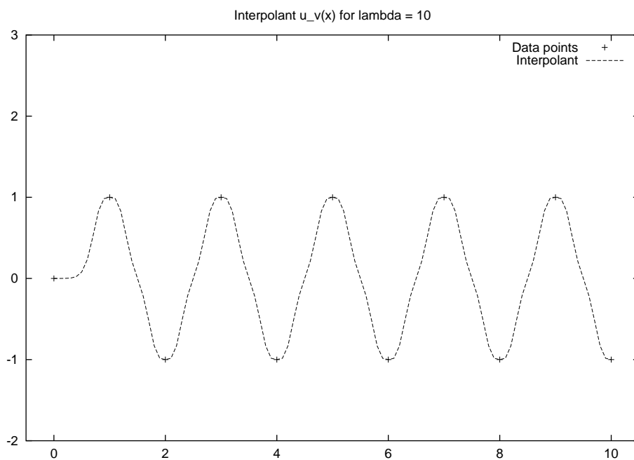
Figure 5: Behavior of the interpolants u_\lambda(x) of (78) and u_v(x) of (94) in the particular case of the sequence \{u_n\} given by (130); \lambda = 10 , \epsilon = 0.01 .
