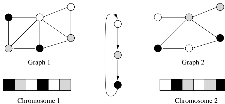
Figure 4: Two solutions with different genotypes and same phenotype, and the swap operation from the first to the second
