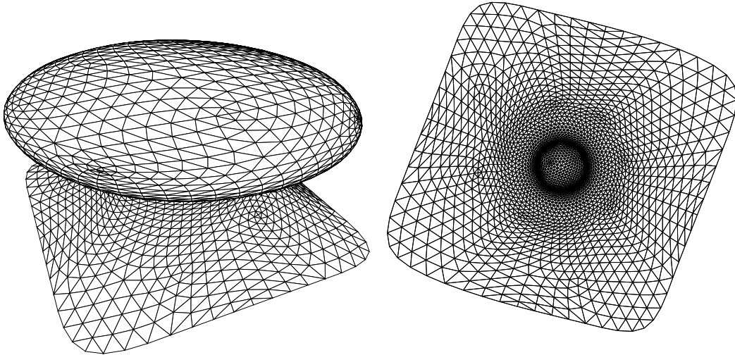
Figure 12: Original mushroom model to resample and its boundary-free parameterization on a disk-like domain.
