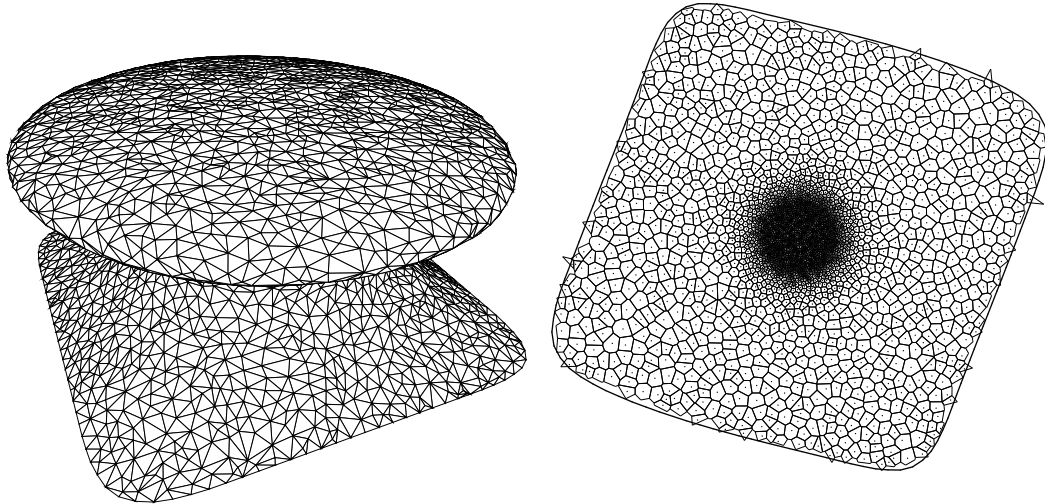
Figure 14: First iteration of Lloyd algorithm with a variable density coming from the area distortion due to parameterization (1.2 s).
