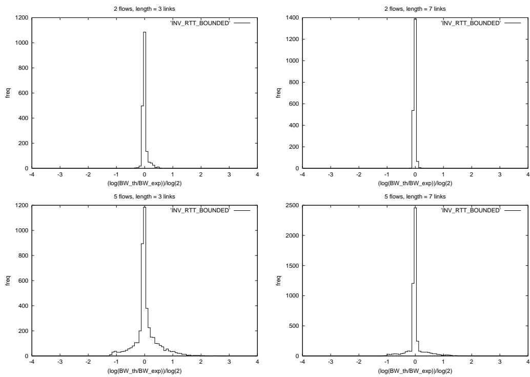
Figure 16: Results of INV-RTT-BOUNDED model.
