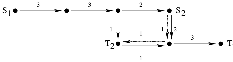
Figure 4: 2-commodity flow from (s_1, s_2) to (t_1, t_2) of value (3, 1)
