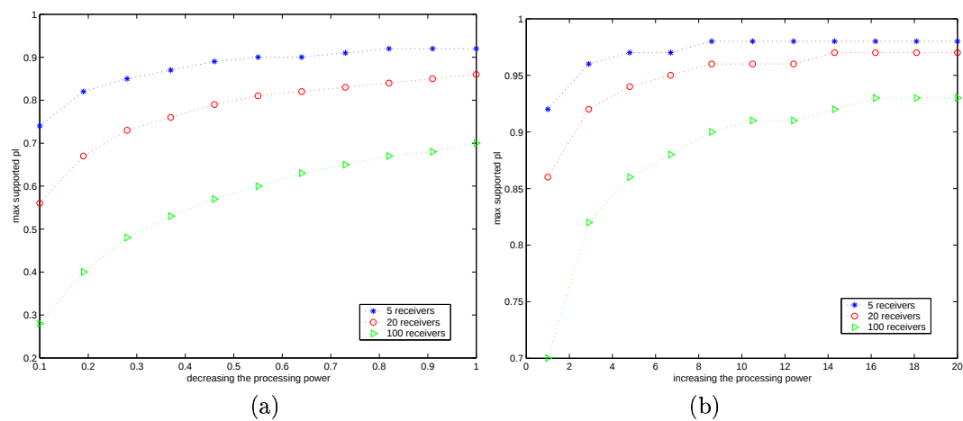
Figure 20: Maximum p_l supported by D as a function of the routers processing power.
