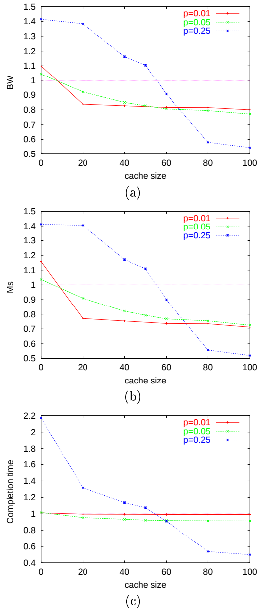
Figure 7: DyRAM vs. ARM (a) Consumed bandwidth, (b) Load at the source, (c) Completion time.
