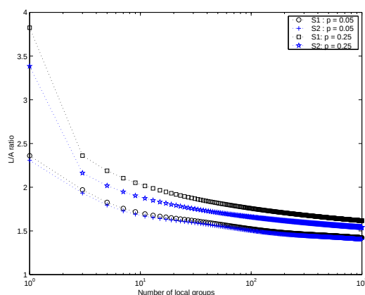
Figure 19: Receiver to active router throughput ratio. B = 10 and 50% of active routers.
