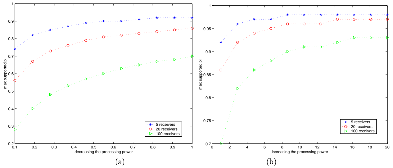
FIG. 6 – Maximum p_i supported by D as a function of the routers processing power.
