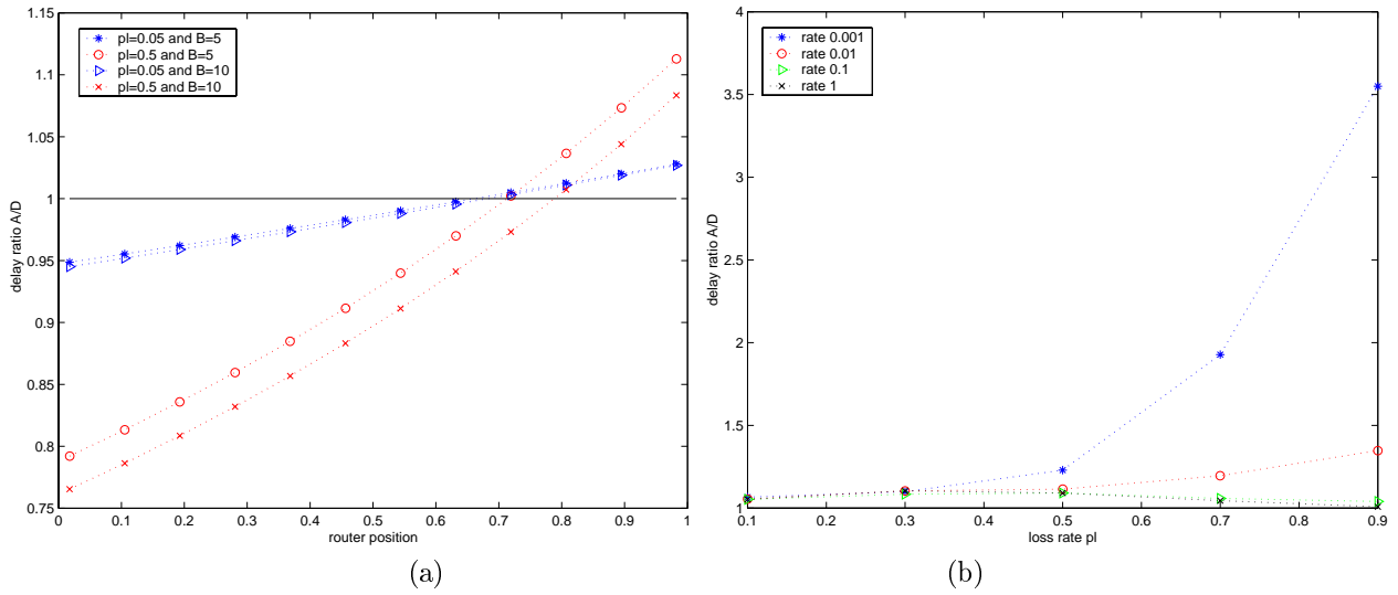
FIG. 4 – The delay ratio A/D as a function of (a) the router position (b) loss rate p_l .
