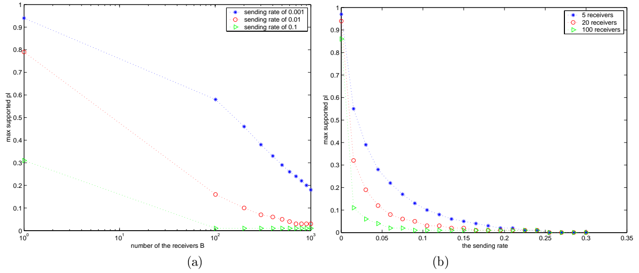
FIG. 5 – Maximum supported p_i in D as a function of (a) B , the number of the receivers and (b) \lambda , the sending rate.
