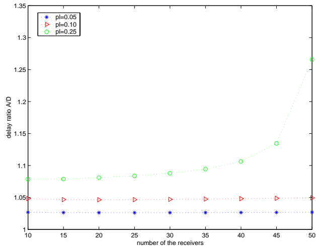
FIG. 9 – The gain for \lambda = 0.01 with B = 5 .
