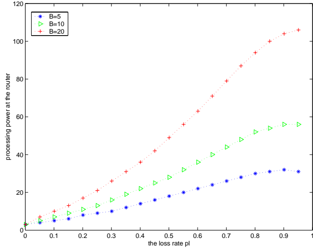
FIG. 7 – The required processing power at the router.
