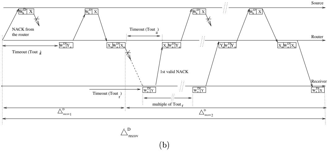
Figure 2: Overall delay diagram for protocol (a) A and (b) D .
