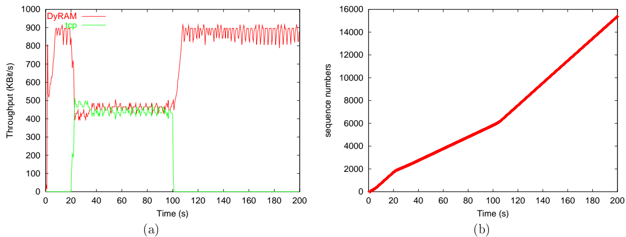
FIG. 8 – Dynamic behavior of DyRAM with one TCP flow
