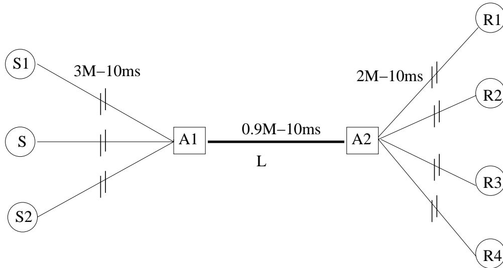
FIG. 5 – The used topology
