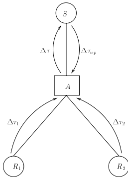
FIG. 4 – CRs aggregation in a multicast tree
