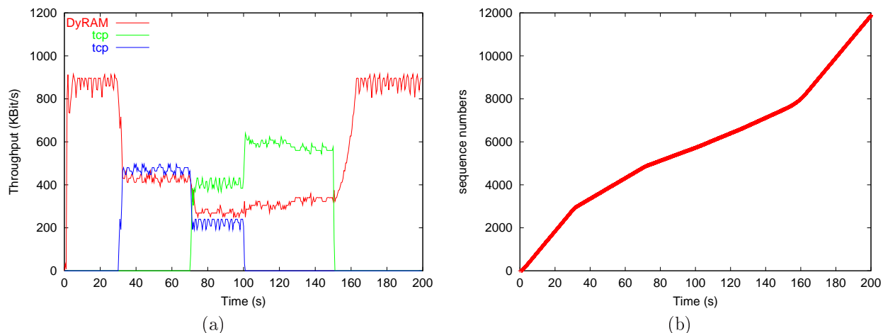
FIG. 9 – Dynamic behavior of DyRAM with two TCP flows
