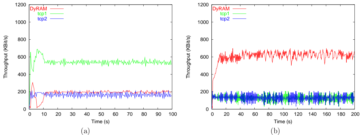
FIG. 11 – Multiple bottleneck links : (a) R1,R4(2M),R2,R3(0.2M), (b) R1,R2(2M), R3,R4(0.2M)
