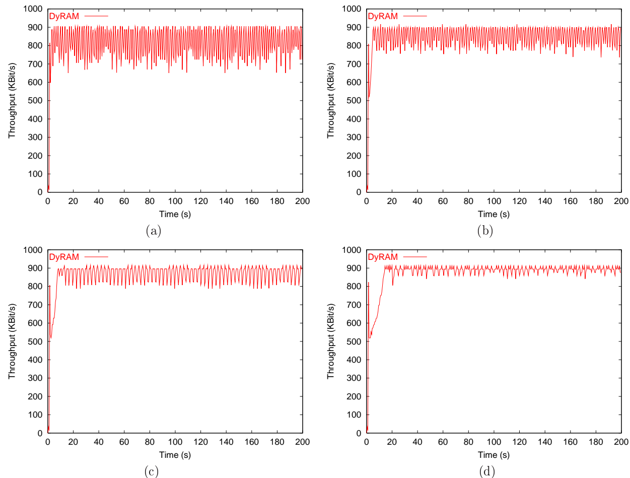
FIG. 6 – The tradeoff between responsiveness and stability (a) 16, (b) 32, (c) 64, (d) 128
