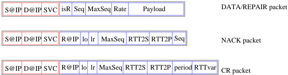
FIG. 1 – Packets structure.
