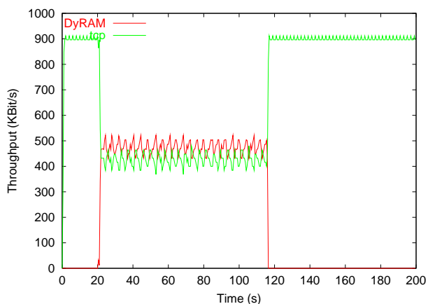
FIG. 10 – Fairness with one TCP flow in the background
