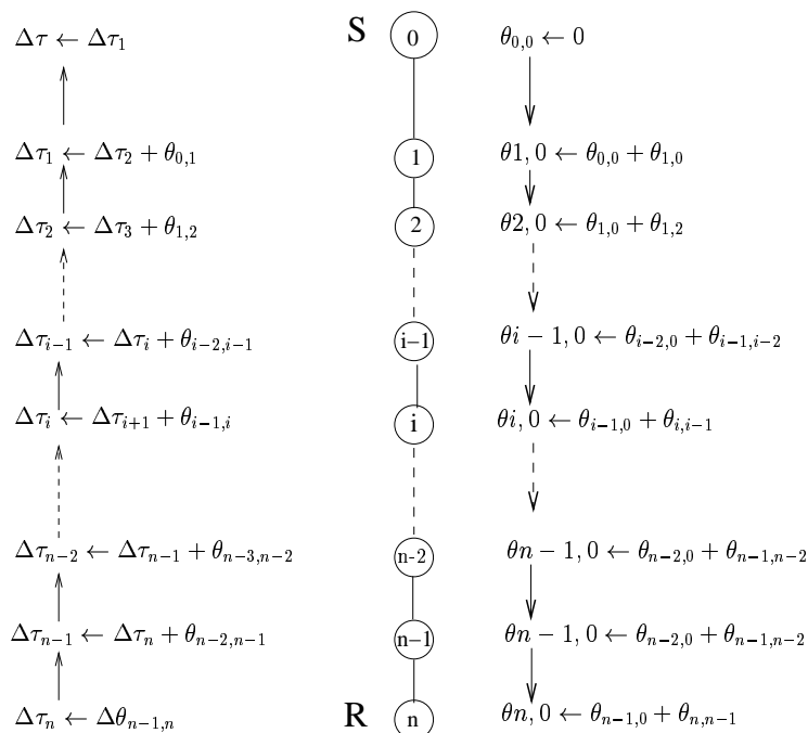
Figure 3: RTT estimation and CRs aggregation
