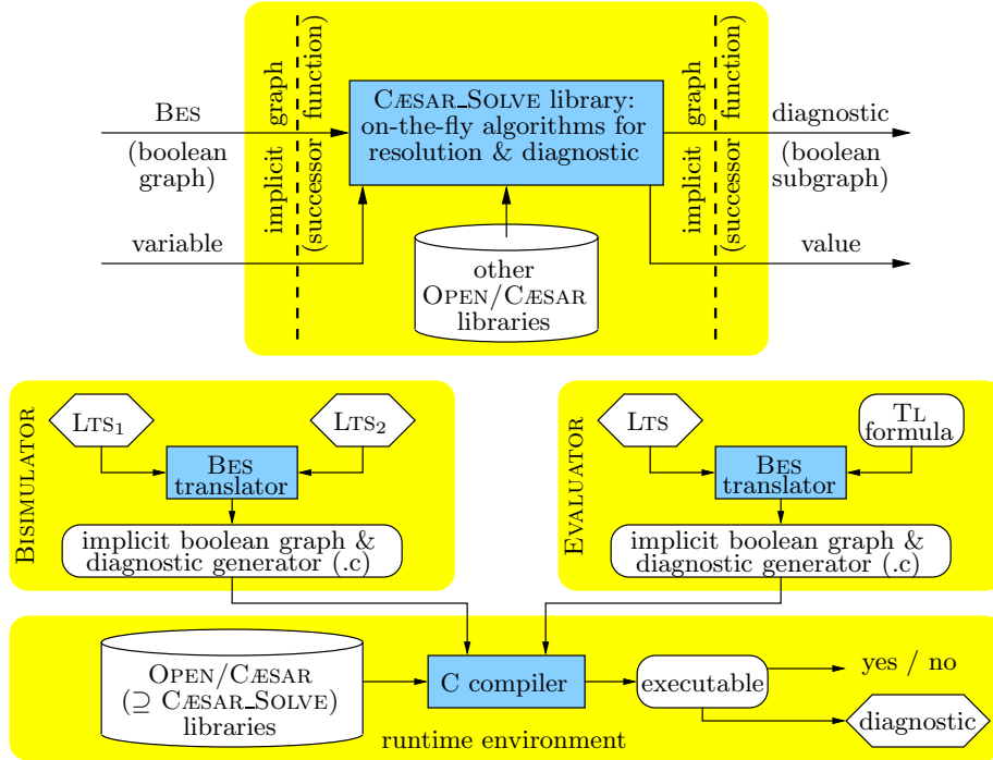
Figure 3: The CÆSAR_SOLVE library and the tools BISIMULATOR and EVALUATOR
