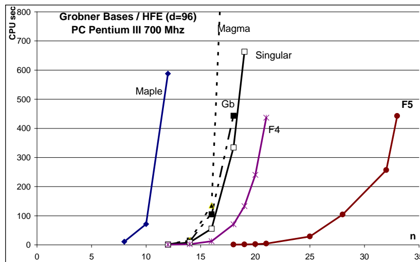
Comparison of various algorithms and implementations (PC PIII 700 Mhz)
