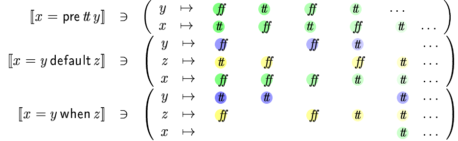
Figure 5: Delay, sampling and merge
