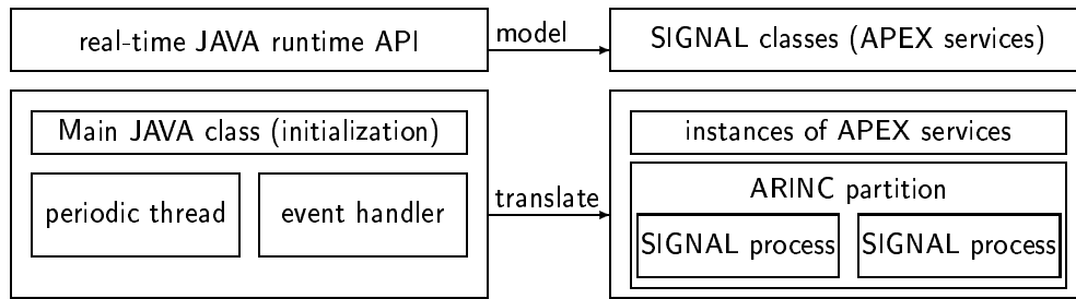
Figure 7: Architecture of the real-time JAVA plugin for POLYCHRONY
