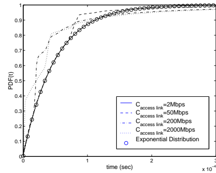
Figure 11: Bottleneck 100Mbps, 100 access links, Pareto file size, load 0.9, average file size 30KBytes
