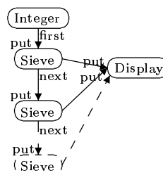
Figure 4: Sieve of Eratosthenes (push)
