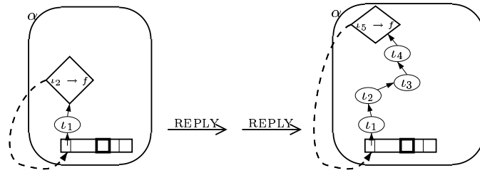
Figure 14: Equivalence in case of cycle of futures
