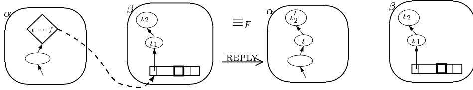
Figure 12: Simple example of future Equivalence
