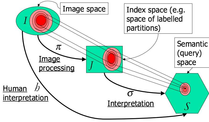
Figure 2: Database schema
