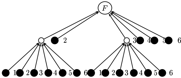
Figure 3: Proof tree for the abstract train controller
