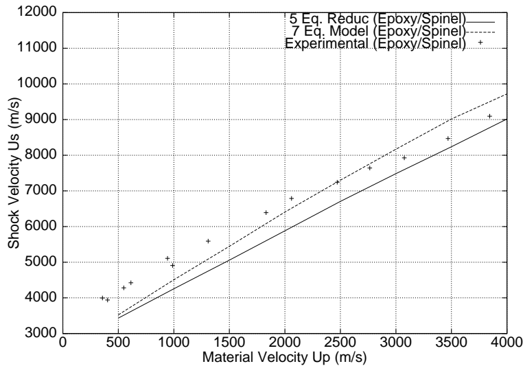
Figure 9: 5 equation reduced model (solid line) and 7 equation model (dotted line) in the Mixture Hugoniot (epoxy/spinel) problem and experimental data (symbols).
