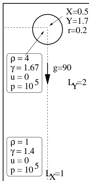
Figure 10: Initial configuration for the first two dimensional test : bubble drop.
