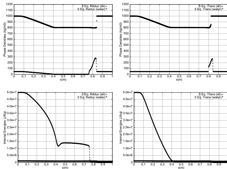
Figure 4: 5 equation reduced model (left) and 5 equation transport model (right) in the water-air shock tube : phase variables. Computed solutions with 1000 cells (symbols).
