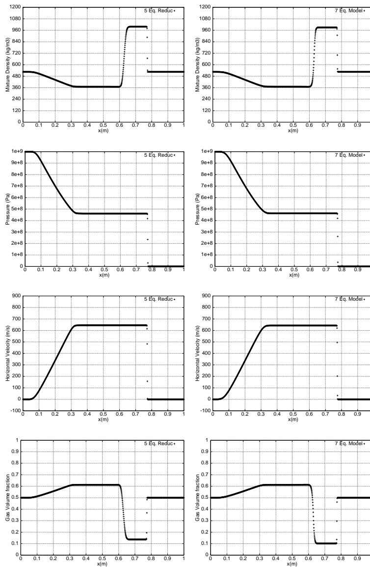
Figure 5: 5 equation reduced model (left) and 7 equation model (right) in the first two-phase flow problem. Computed solutions with 1000 cells (symbols).
