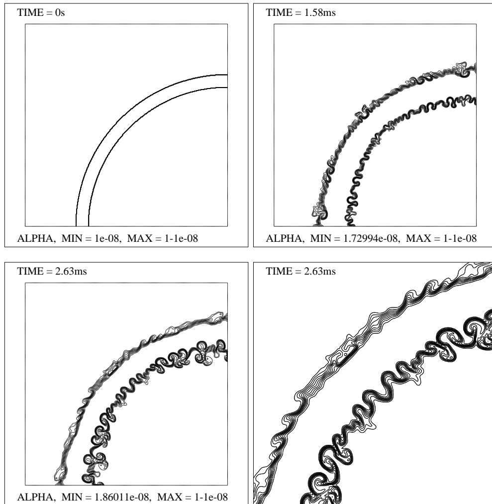
Figure 13: Isovalues of the volume fraction for the second two dimensional test.
