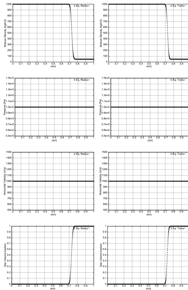
Figure 2: 5 equation reduced model (left) and 5 equation transport model (right) in the pure interface advection : mixture variables. Computed solutions with 1000 cells (symbols).
