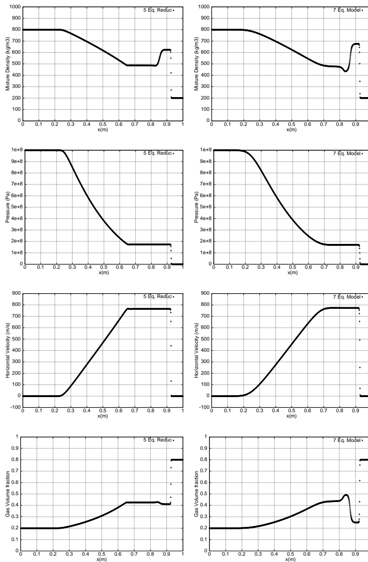
Figure 6: 5 equation reduced model (left) and 7 equation model (right) in the second two-phase flow problem. Computed solutions with 1000 cells (symbols).
