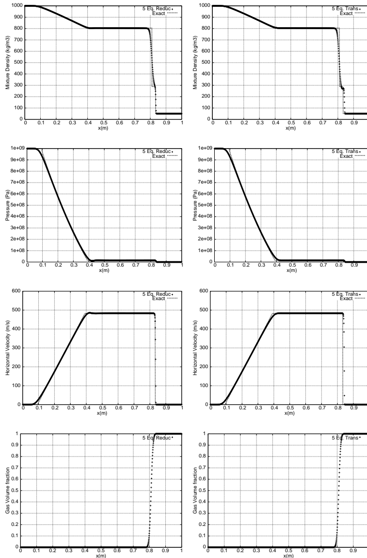
Figure 3: 5 equation reduced model (left) and 5 equation transport model (right) in the water-air shock tube : mixture variables. Computed solutions with 1000 cells (symbols) and exact solutions (dotted lines).
