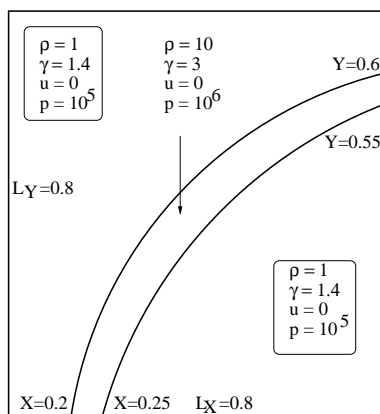
Figure 12: Initial configuration for the second two dimensional test.
