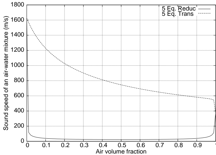
Figure 1: Sound speed of an air-water mixture under atmospheric conditions for the 5 equation reduced model (solid line) and the 5 equation transport model (dotted line).
