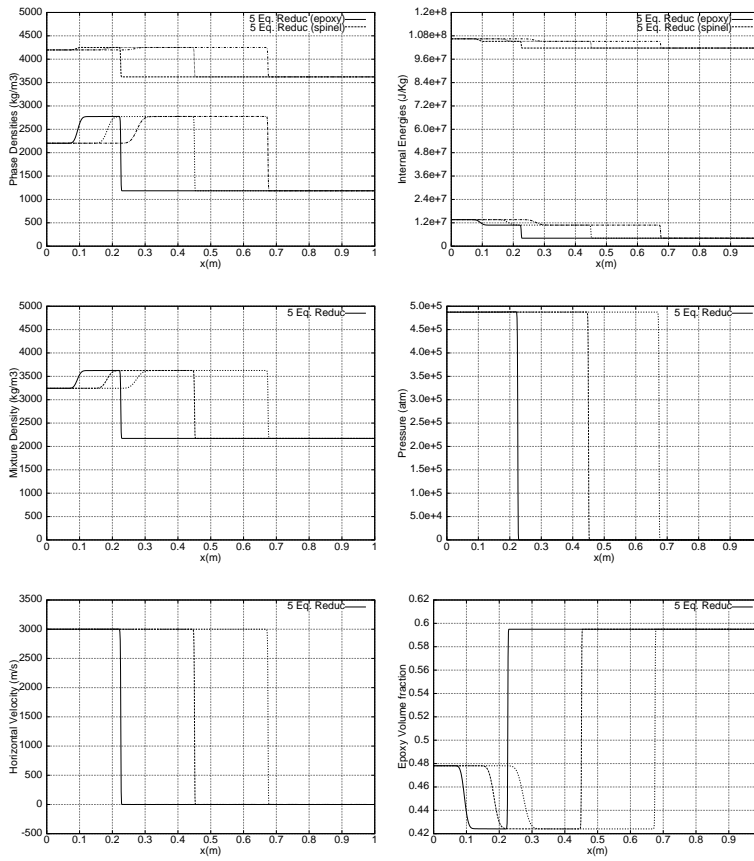
Figure 8: Results of the 5 equation reduced model for the epoxy/spinel under shock impact at 3000m/s. Computed solution with 1000 cells.
