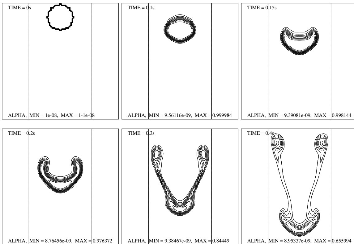
Figure 11: Isovalues of the volume fraction for the first two dimensional test : bubble drop.
