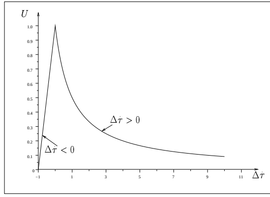
Figure 2: The inter-receiver fairness as a function of the relative RTT variation.
