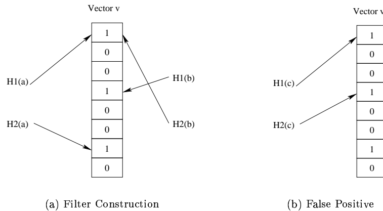
Figure 1: Bloom Filter
