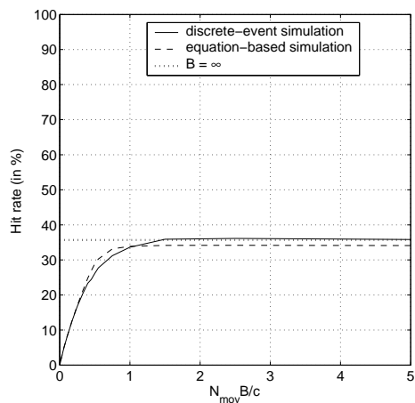
Figure 6: Impact of B on the hit rate.
