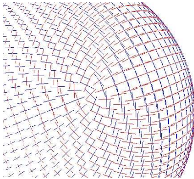
Figure 18: Elliptic paraboloid
