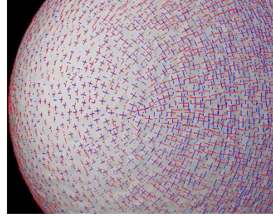
Figure 23: Principal directions on a noisy ellipsoid
