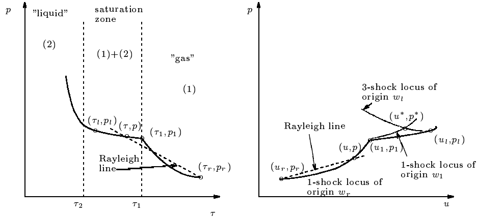
FIGURE 4.1. Non-uniqueness of the Riemann problem
