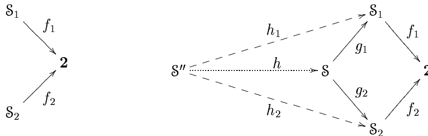
Figure 6: The interface of synchronisation and the pullback
