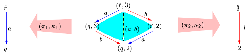
Figure 8: A product of asynchronous systems in the category with flat morphisms.
