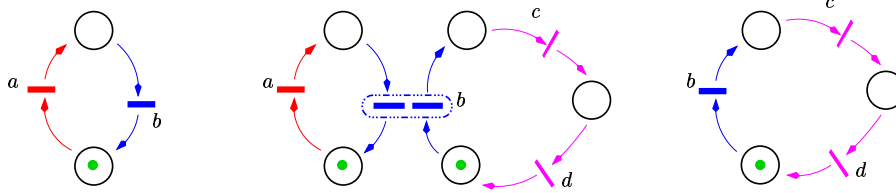
Figure 1: Decomposition of an elementary net into sequential components.
