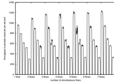
Figure 10: Measured throughput in the growing number of contending flows experiment
