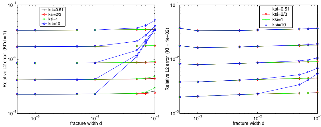
Figure 6: Test case 1. Discrete relative L^2 error variation as a function of the fracture width d , for different values of \xi . \xi = 0.51 in black, \xi = 2/3 in red, \xi = 1 in green, \xi = 10 in blue. The five sets of curves show the dependency over the mesh size. From the upper curves to the lower ones: h = 1/10 , h = 1/20 , h = 1/40 , h = 1/80 , and h = 1/160 . Left: the fracture permeability varies as 1/d . The permeability increases as the fracture width decreases: K_f \times d = 1 . Right: the fracture permeability is constant: K_f = 100 .
